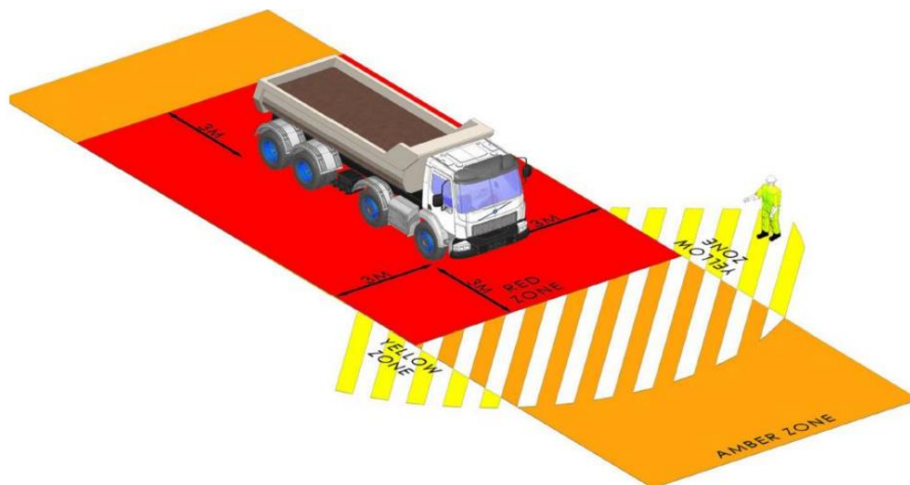
Gambar 16. Zona Keselamatan Dump Truck
