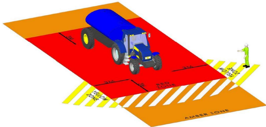
Gambar 22. Zona Keselamatan Water Tank Truck
