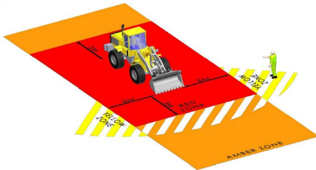
Gambar 24 Zona Keselamatan Wheel Loader
